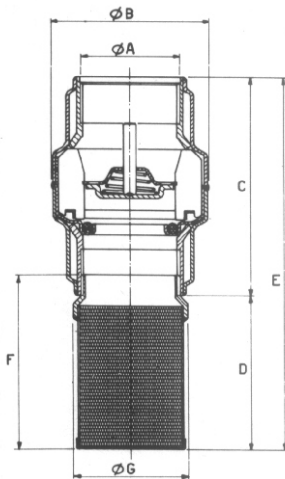
Art. 077.0001 with stainless steel grasping rack
